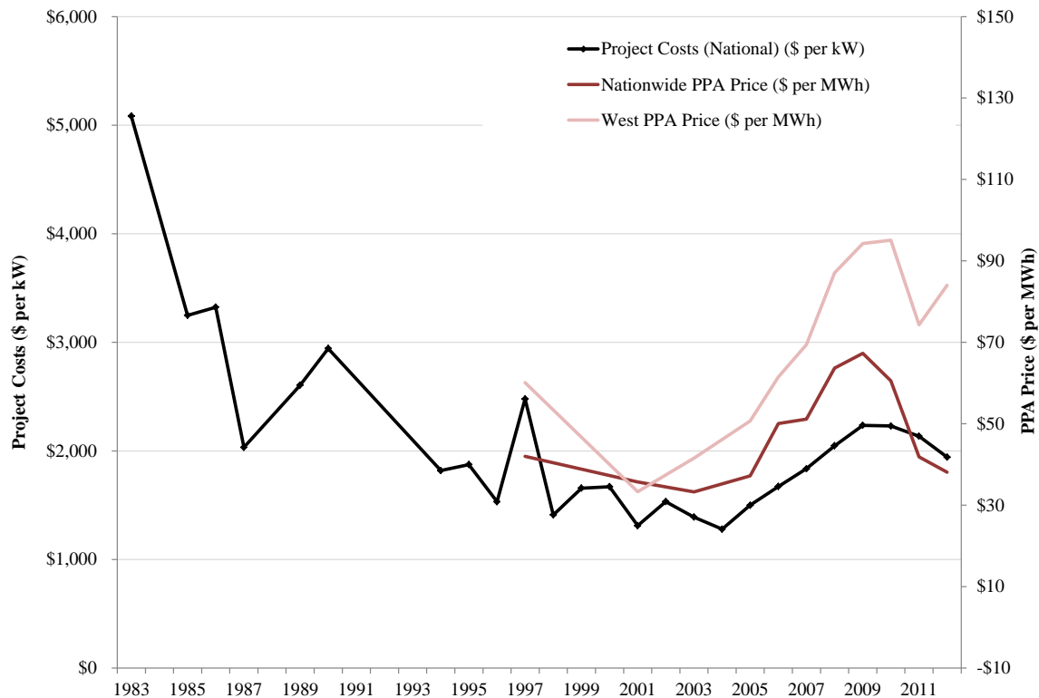
Figure 4. Wind Power Project Costs ($ per kW) and Purchase Power Agreement Prices ($ per MWh)
