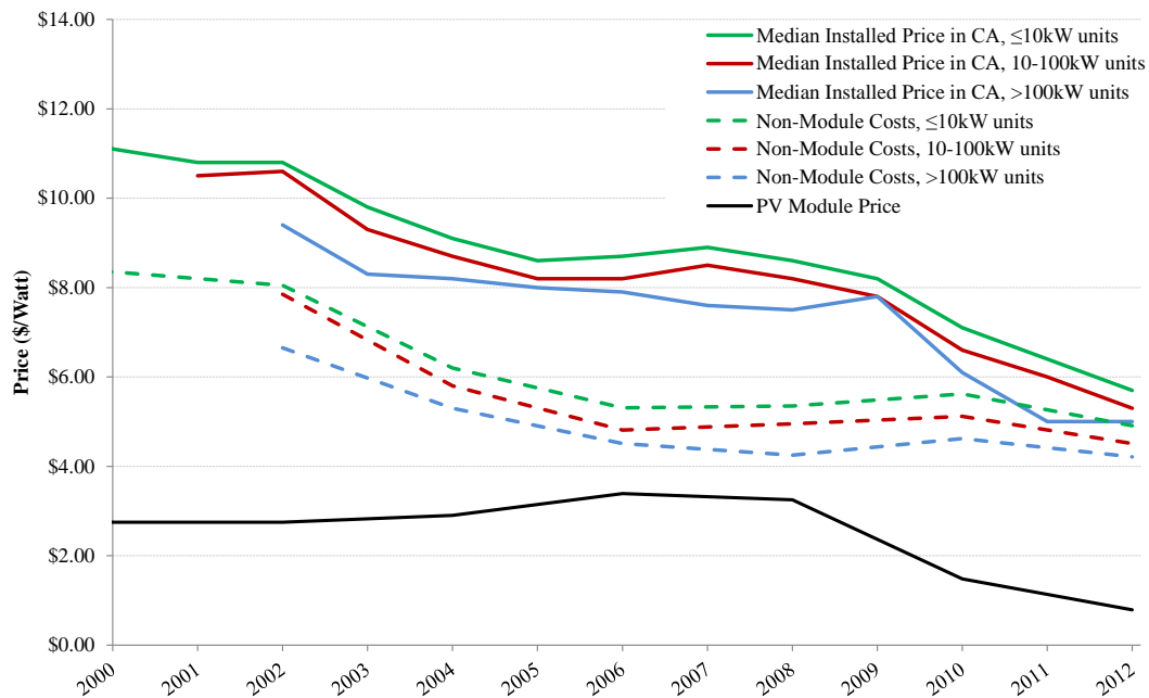
Figure 3. Solar Photovoltaic Costs
